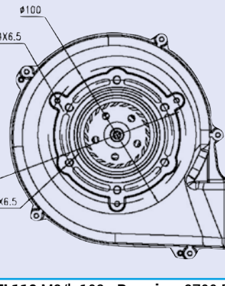
Type FL118 M3/h 102 - Pression: 2700 Pa
