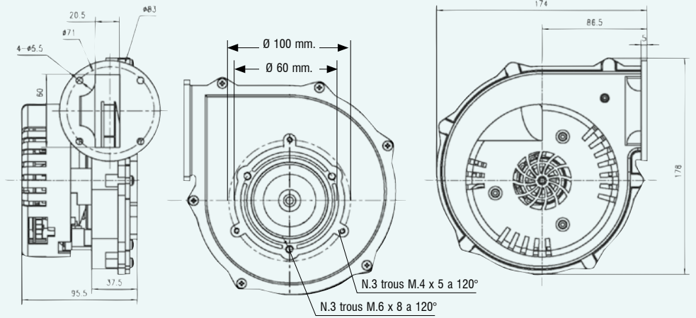
Type FL130 m 3 /h 125 Pression: 2500 Pa
