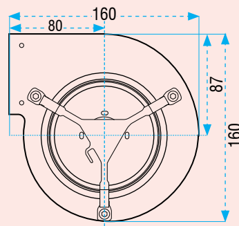
Art. N.643.00 - Centrifugal fan, double aspiration TRIAL type CAD 12R-001 with air vent 146 x 63.3.
