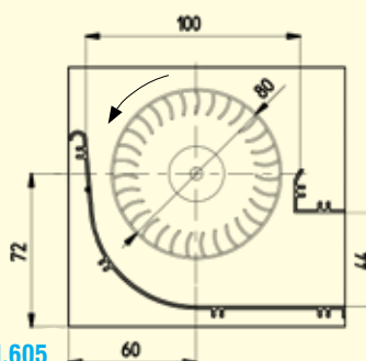
Art. N.605 - FERGAS tangential fan for high-temperature, motor positioned on the left. Voltage 230 V 50 Hz.
