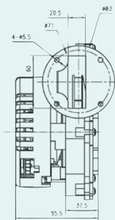
Type FL130 mc/h 125 Pressure: 2500 Pa
