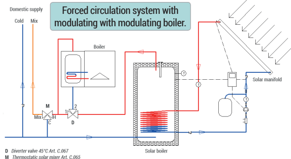
AN EXAMPLE OF ILLUSTRATED INSTALLATION SCHEME
